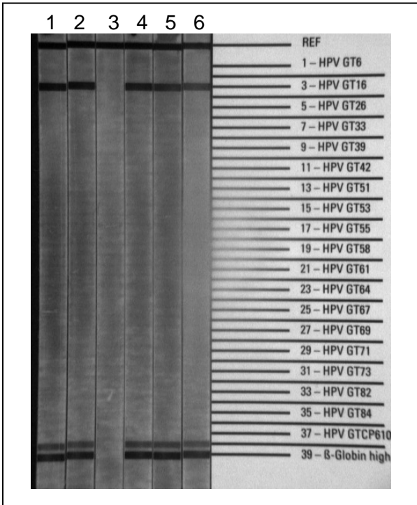
Fig. 1. Use of Roche Linear Array to detect HPV DNA (subject Samples in lanes 1, 2, 4-6). Lane 3 was a negative control (no DNA).
